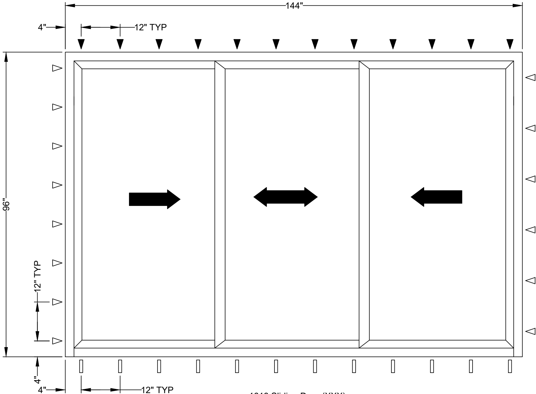
1618 Sliding Door (XXX) Maximum Size: 144" x 96" Design Pressure: +50/-50 psf Missile D - Wind Zone 3
